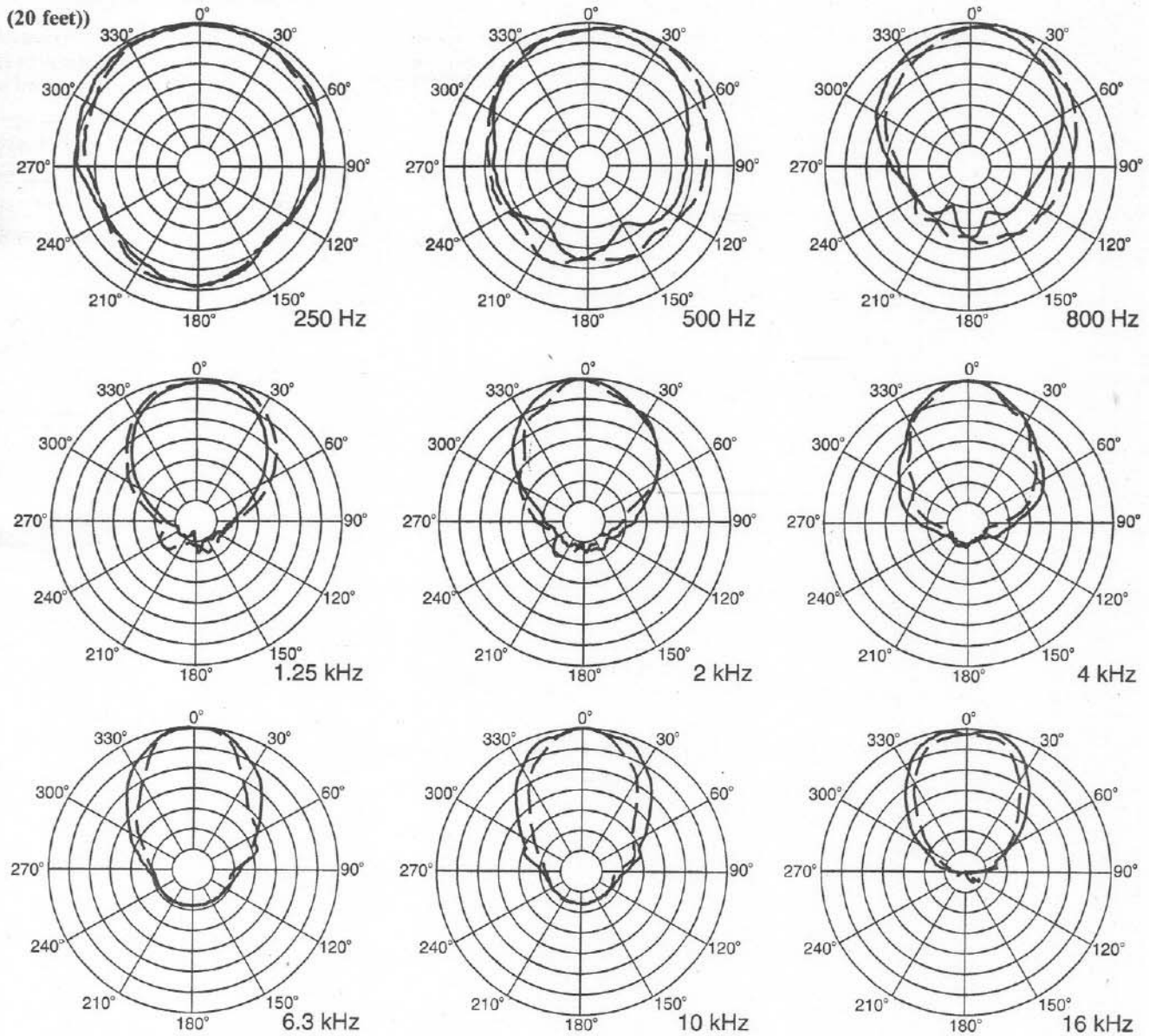
Figure 6—T15i Beamwidth vs. Frequency (anechoic environment)
